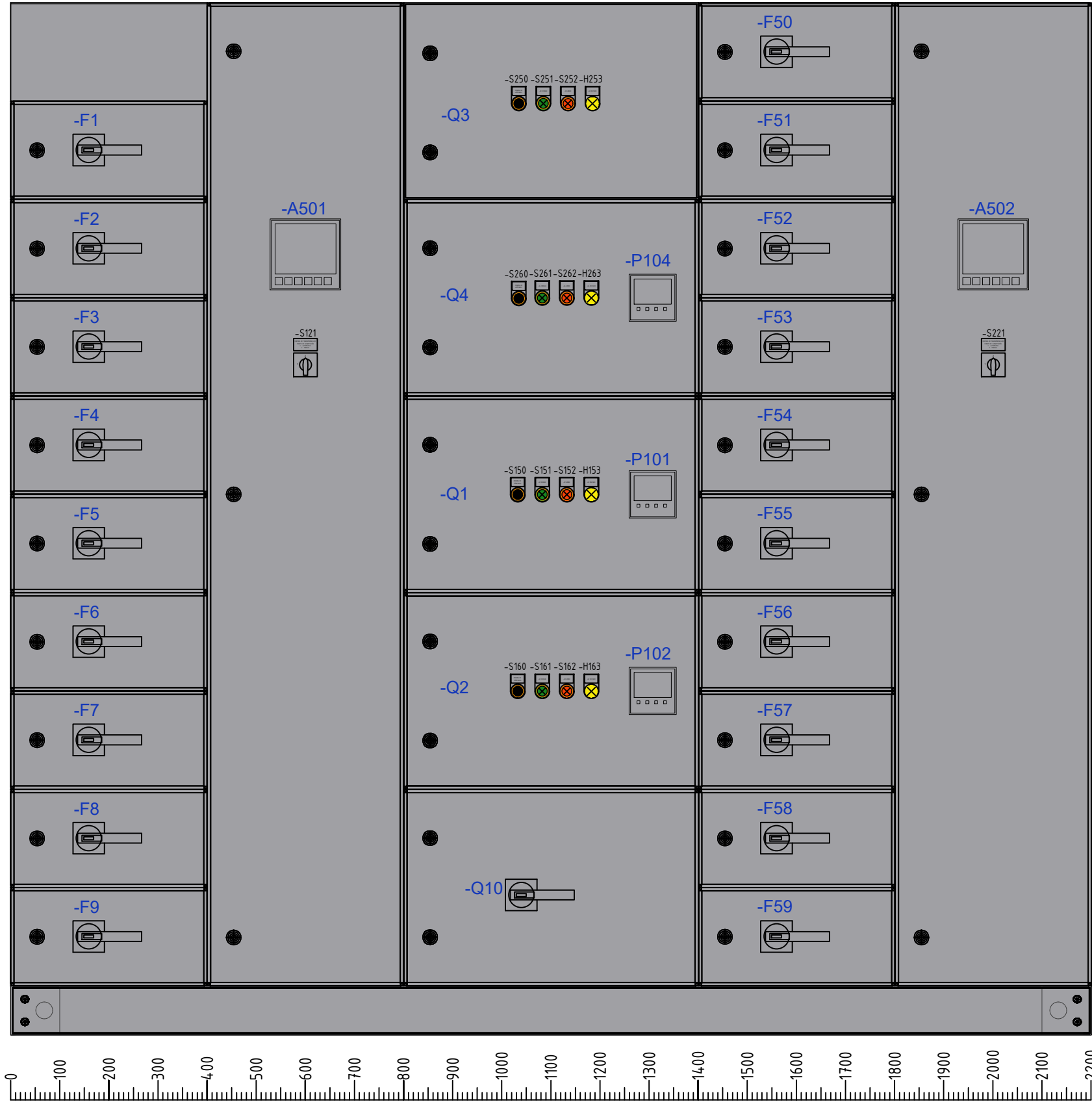
VISTA FRONTAL
